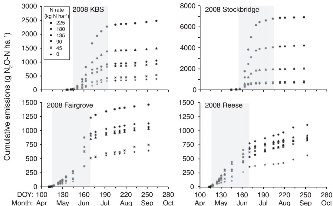
Fig. 2 Cumulative N_2O emissions during the 2008 growing season. The shaded portion of the graph represents the 47–54-day period where daily flux for the N treatments was greater than the control treatment ( \geq 4 \text{ g } N_2O \text{ ha}^{-1} \text{ day}^{-1} ).
