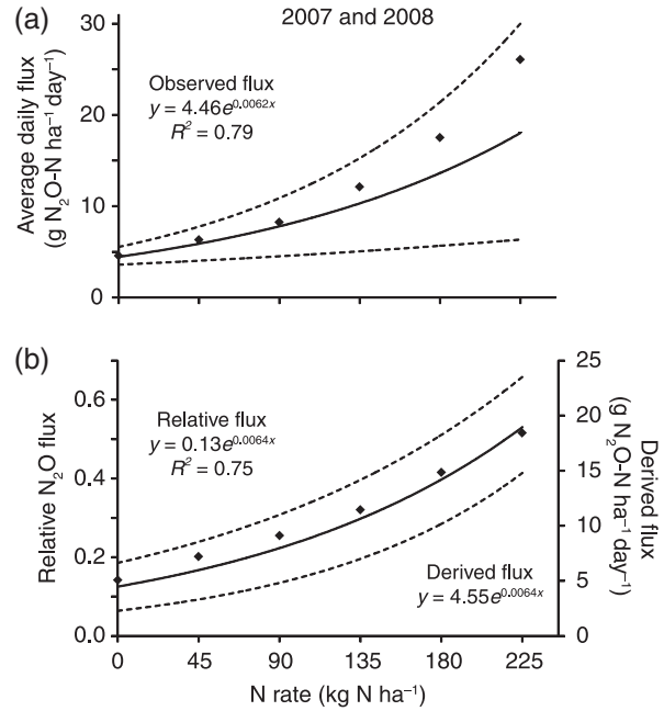
Fig. 6 Results from regression analysis using site averages for each N rate. (a) The model curve for the average daily flux is shown with the observed averages. (b) The relative flux model was used to calculate the derived flux using model predictions and the observed flux for 0 kg N ha -1 at each site to back-calculate a scaled value (kg N 2 O–N ha -1 yr -1 ). The 95% confidence intervals are shown only for the observed and relative flux model predictions [Eqn (2)].
